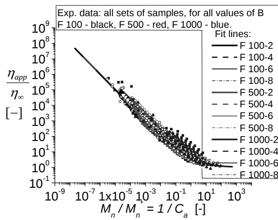
Fig. 13 – Master curve \frac{\eta_{app}}{\eta_{\infty}} = f\left(\frac{M_n}{M_n^*} = \frac{1}{C_a}\right) obtained for different values of magnetite and Fe
