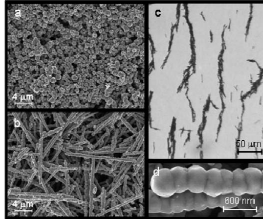
Fig. 3 – SEM images of: a) spheres ( 680 \pm 150\text{ nm} ); b) magnetite rods (sizes 560 \pm 120\text{ nm}/6900 \pm 3800\text{ nm} ) dispersed in MRFs; c) typical structure induced in MRFs containing microrods by magnetic fields; d) magnetite microrods detail [86]. Reprinted from de Vicente J., Segovia-Gutiérrez J.P., Andablo-Reyes E., Vereda F. (2009), Dynamic rheology of sphere- and rod-based magnetorheological fluids , The Journal of Chemical Physics 131 (19), 194902; doi:
