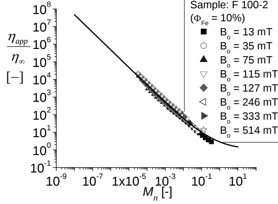
Fig. 12 – Dimensionless viscosity as a function of Mason number, \frac{\eta_{app}}{\eta_{\infty}} = f(M_n) , for sample
