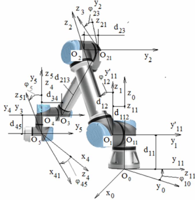
Fig. 7 – The necessary notations for solving the direct kinematics with the method of homogeneous operators.
