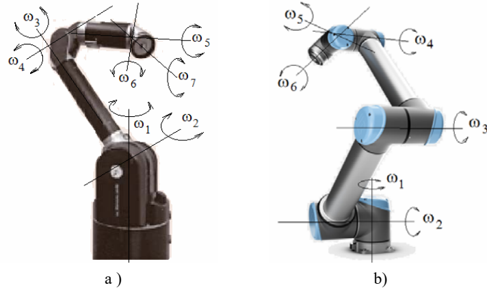
Fig. 2 – Collaborative robots: a) WAM Barrett robotic arm; b) universal robot UR 10 robotic arm.
