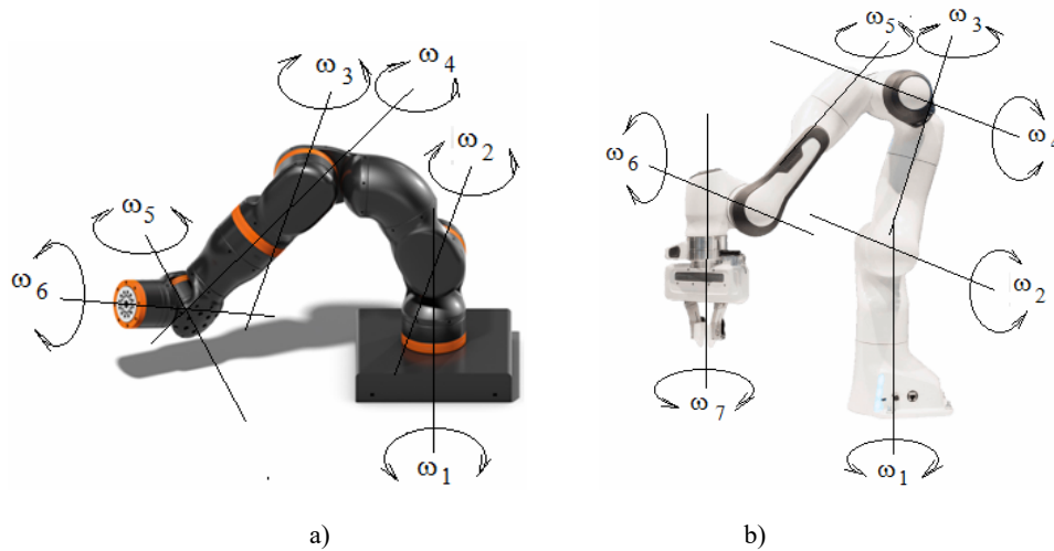
Fig. 5 – Collaborative robots: a) Rebel robotic arm; b) Panda robotic arm.
