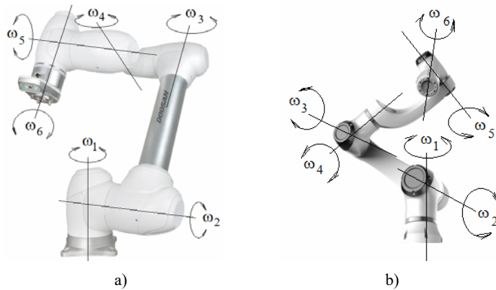
Fig. 3 – Collaborative robots: a) Doosan M 1013 robotic arm; b) Elfin robotic arm.
